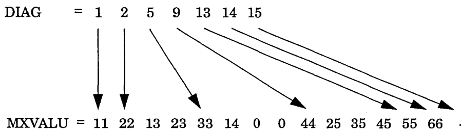
Figure 8-2 Skyline Matrix Representation
