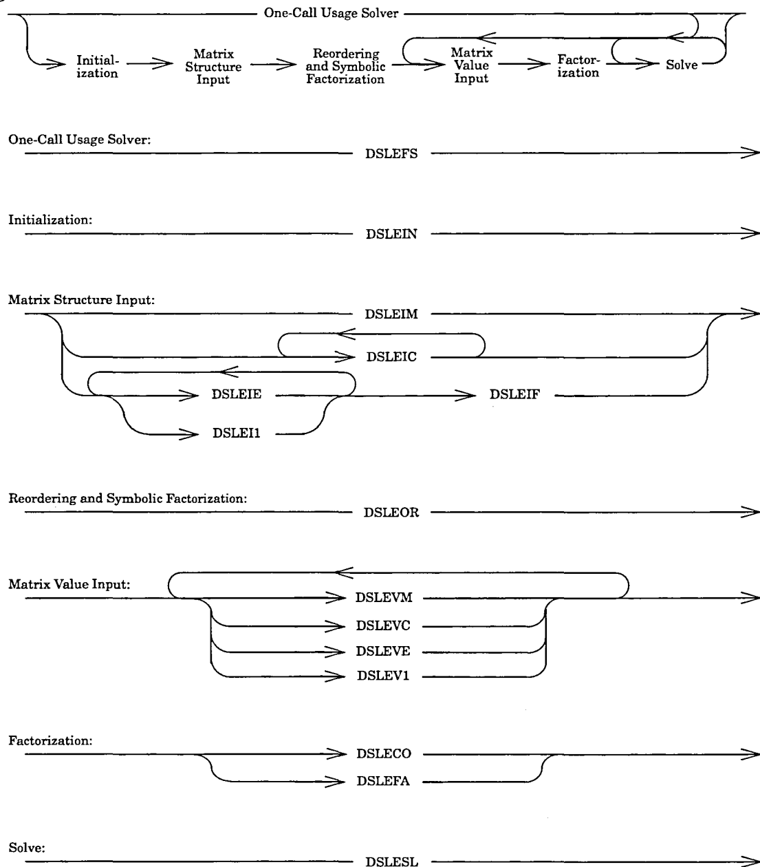
Figure 6-3 Paths of Control
