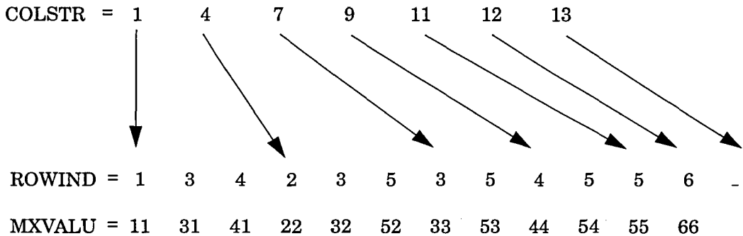
Figure 6-2 Column Pointer, Row Index Sparse Matrix Representation
