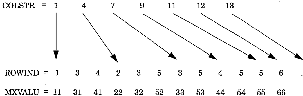
Figure 8-4 Column Pointer, Row Index Sparse Matrix Representation
