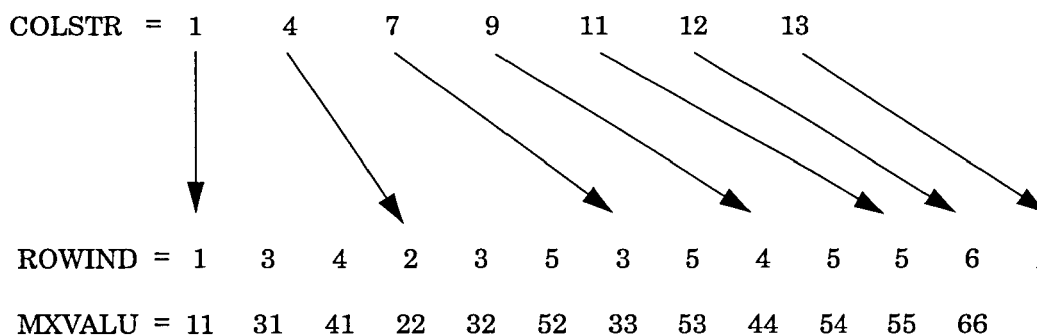
Figure 7-2 Column Pointer, Row Index Sparse Matrix Representation
